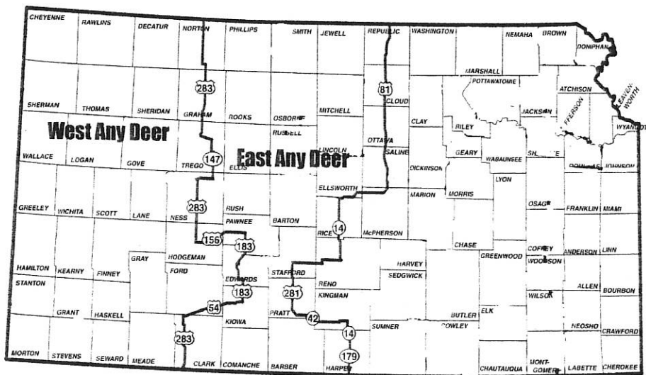
Fig. 4 Draft Any-deer Units
