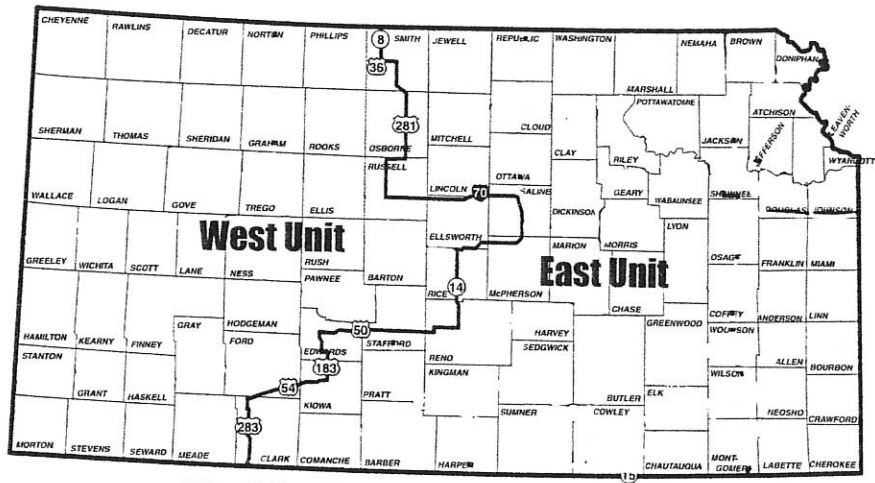
Fig. 3 Draft Whitetail Either Sex Units
