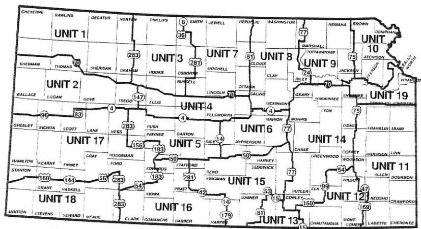
Fig. 2 Current Firearms Deer Management Units
