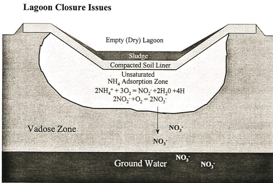
Figure 2. Potential conditions after lagoon closure.
